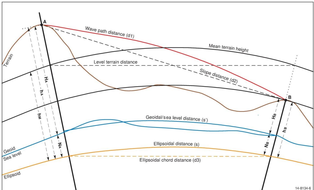
Figure 5.1 Reduction of distance to the ellipsoid.
