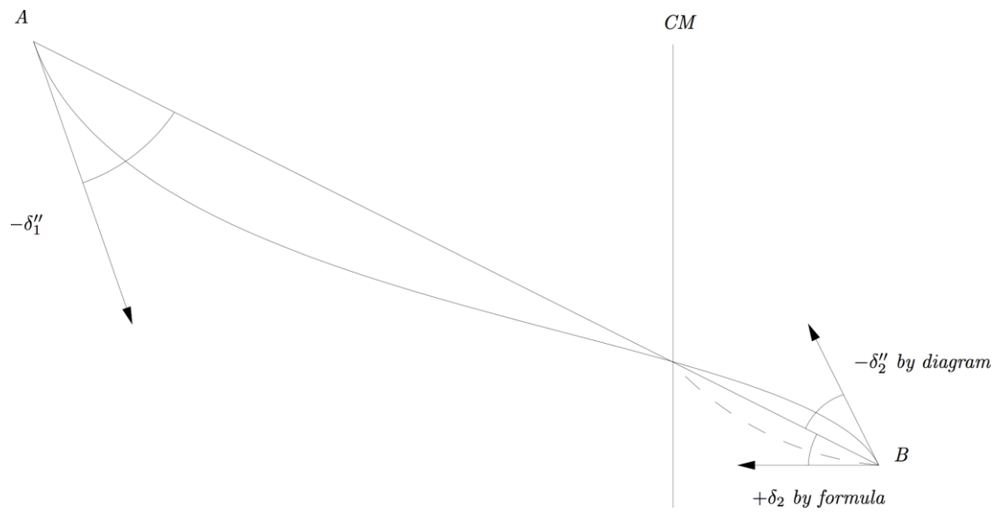
Figure C.1 Arc-to-chord correction
