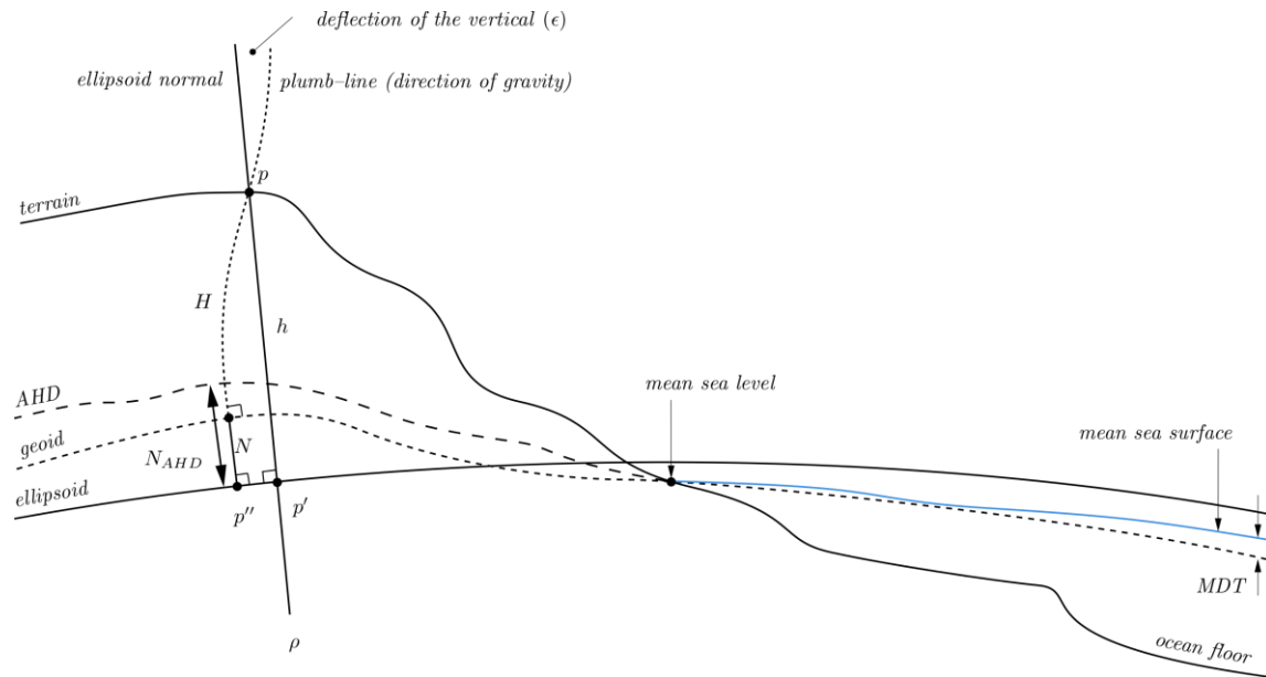
Figure 6.2: Reference and working surfaces for height in Australia.
